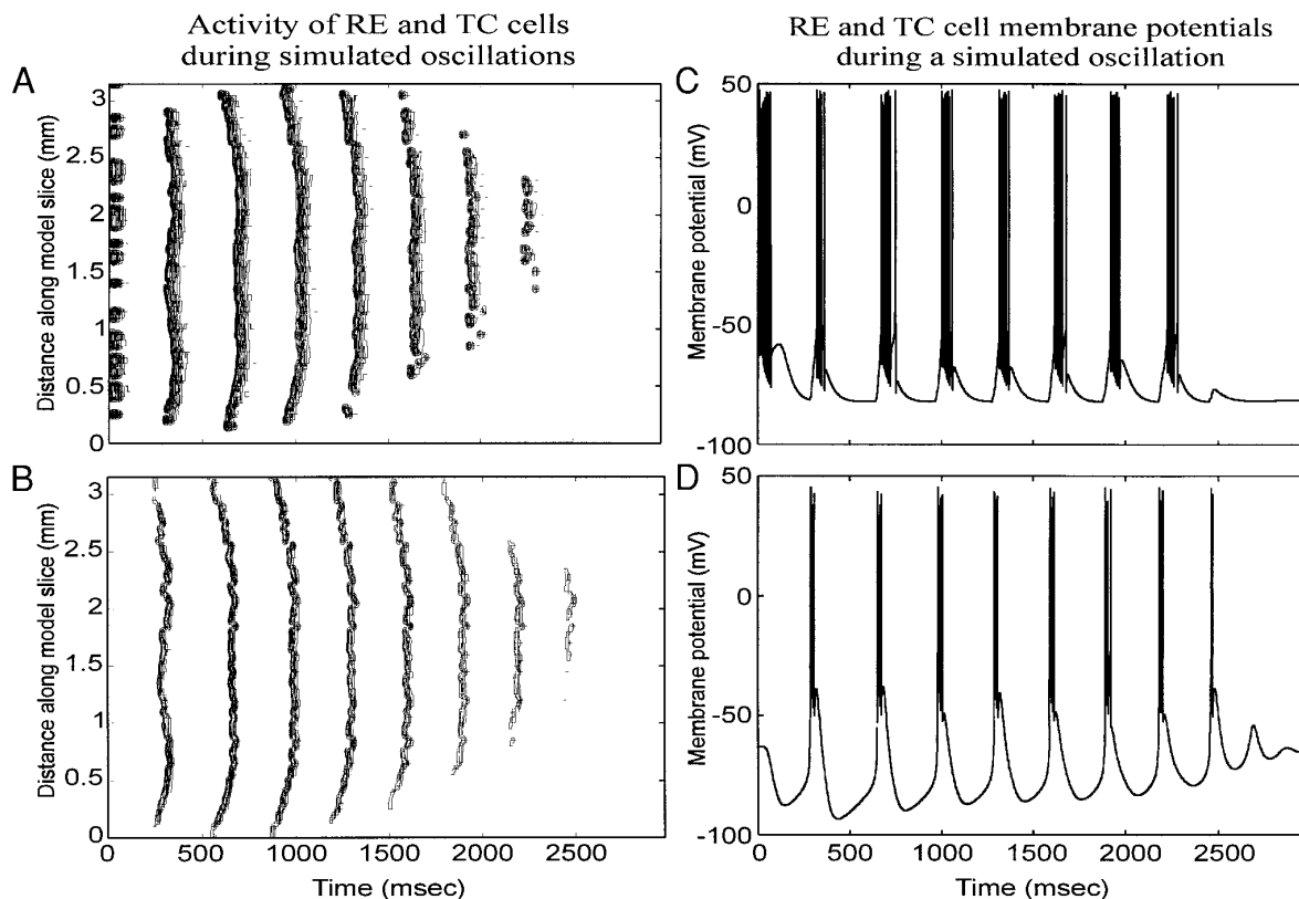
FIG. 2. Synchronous, slow ( \approx 3 -Hz) oscillations in the network model. A : contour plot of the activity of 64 RE cells as a function of time and distance along the model slice. B : similar plot of activity in 64 TC cells. As in Fig. 1, oscillatory activity persisted for \sim 2 s. Activity is expressed as firing frequency. To simulate the indirect excitation of RE cells via stimulation of internal capsule, 1/3 of the RE cells were excited above the burst threshold at time 0 . C : plot of the membrane potential vs. time for an RE cell at the center of the model slice. The RE cell bursts once per cycle, and the number of spikes per burst is similar to that observed during bicuculline-induced slow oscillations in vitro. D : plot of the membrane potential vs. time for a TC cell at the center of the model slice. Again, the TC cell bursts once per cycle, and the number of spikes per burst is similar to that observed in vitro. As the oscillation progresses, GABA release declines because of the activation of presynaptic GABA B autoreceptors on RE cells (not shown). Consequently, the peak deflection of inhibitory postsynaptic potentials (IPSPs) become less hyperpolarized, as observed in vitro, until the IPSPs are too weak to sustain the oscillation. \bar{g}_{\text{GABA-B}} was 30.5 nS [ \bar{g}_{\text{GABA-B}} (tickler) = 21.8 nS and \bar{g}_{\text{GABA-B}} (cluster) = 8.7 nS] and \bar{g}_{\text{AMPA}} was 150 nS.
